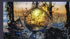
ACID RAIN
